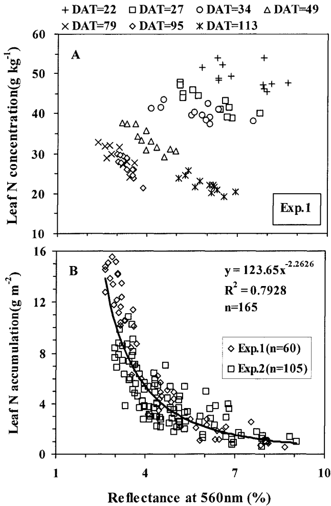
Fig. 2. Relationship of canopy reflectance at 560 nm to (A) leaf N concentration and (B) leaf N accumulation in rice with different N treatments over the growth period. DAT, days after transplanting.
