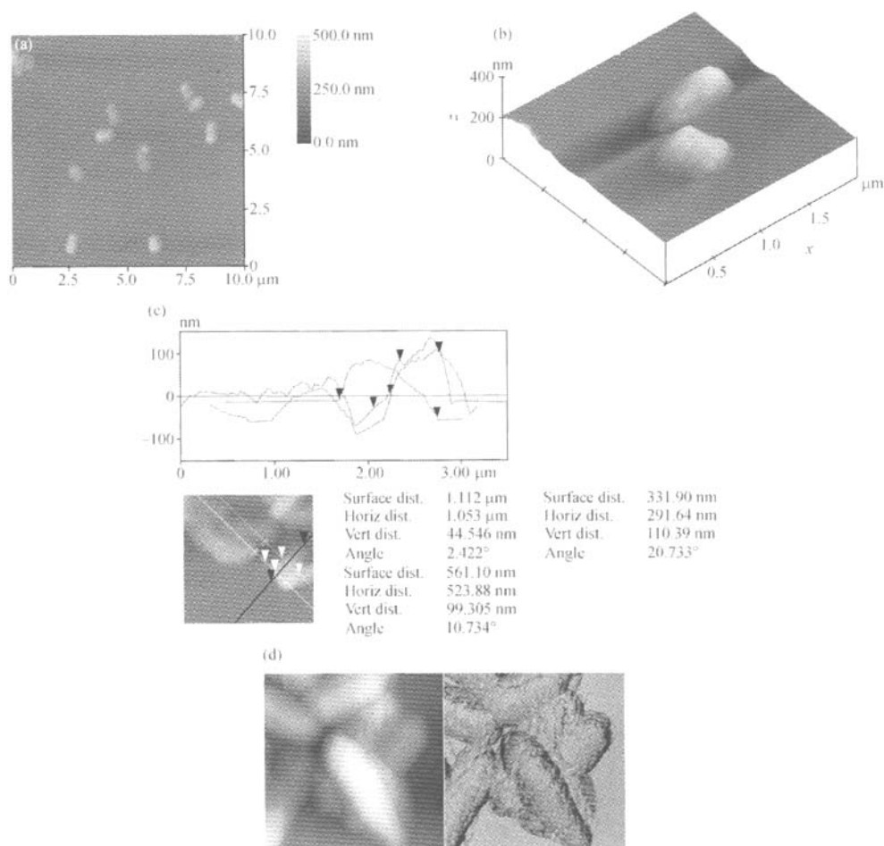
Figure 4 Surface roughness contrast between bare and metallized E. coli cells.
