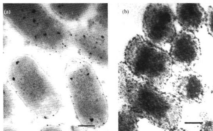
Figure 1 TEM images of bare and metallized bacterial cells. (a) Bare bacterial cells; (b) bacterial cells after Pd (II) activation and subsequent nickel deposition for 30 s; (c) bacterial cells after Pd (II) activation and subsequent nickel deposition for 15 min, the inset image is the electron beam diffraction, the scale bar = 300, 150, 200 nm, respectively; (d) and (e) are the histogram of size distribution of nickel particles from (b) and (c), respectively.
