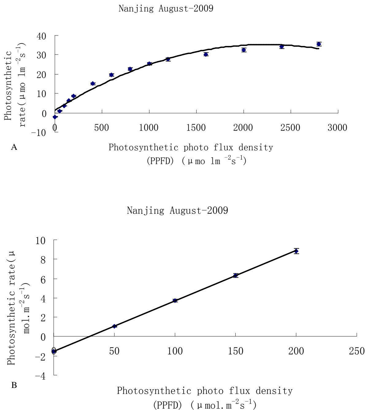
Figure 3. The response curve of PPFD for photosynthesis of the leaves in Eichhornia crassipes
