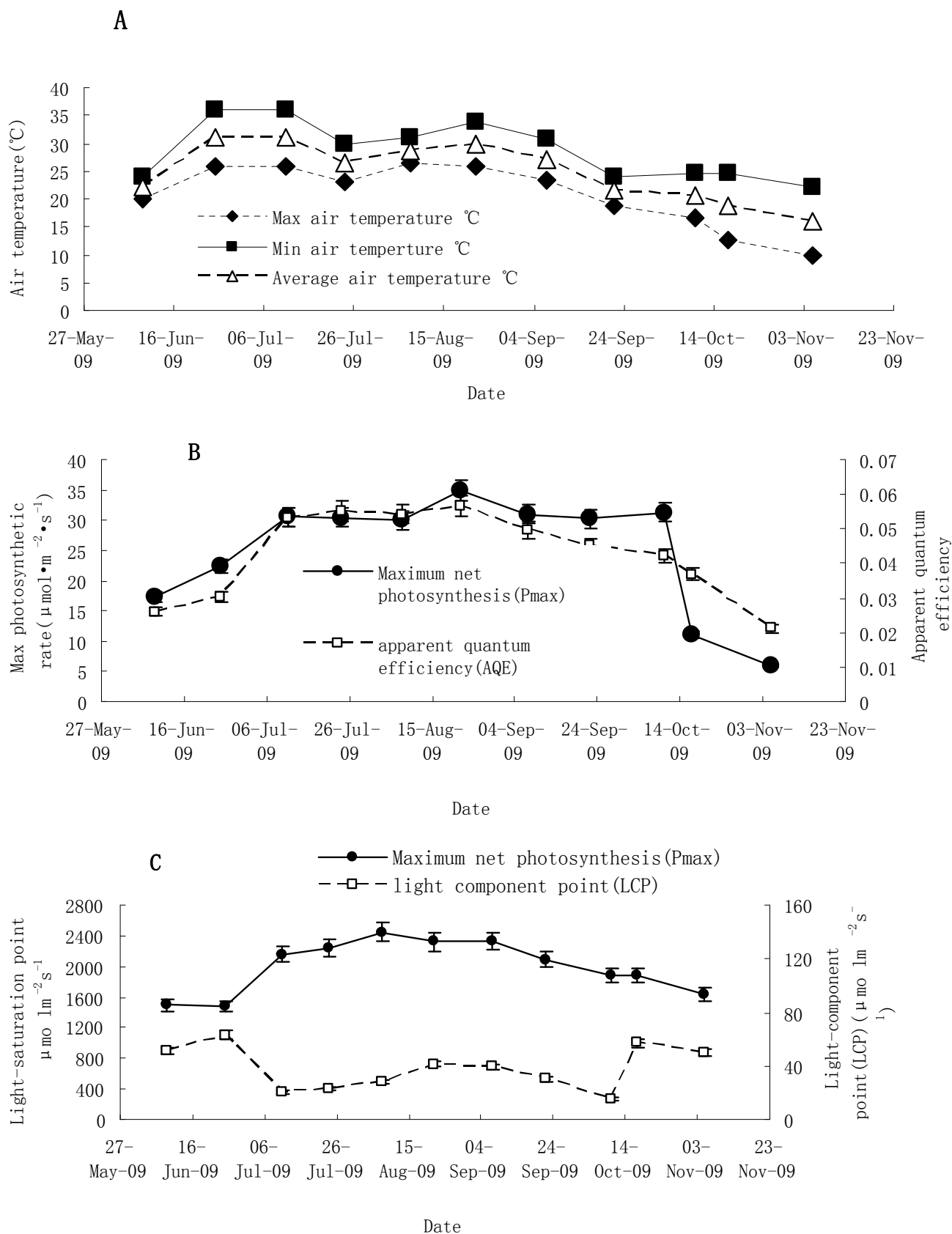
Figure 1. The changes in the maximum net photosynthesis (Pmax), light component point (LCP), apparent quantum efficiency (AQE) and light-saturation point (LSP) of leaves in E. crassipes and the air temperature of this period in natural conditions.
